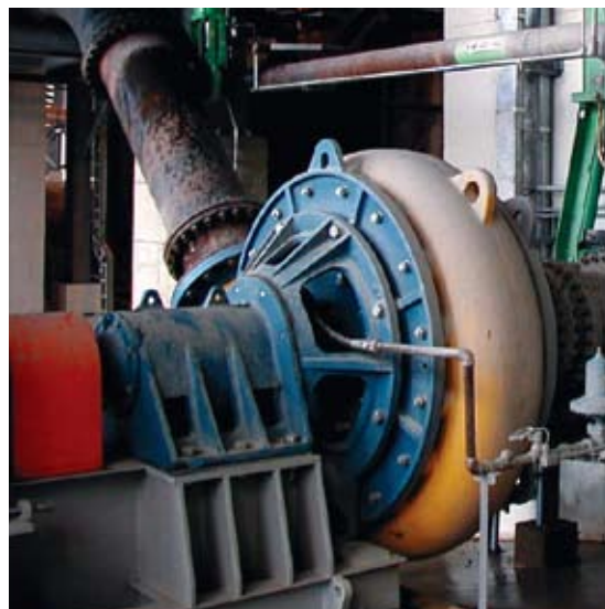
Left: Cover plate of a 550 MCR to be installed at a copper plant
